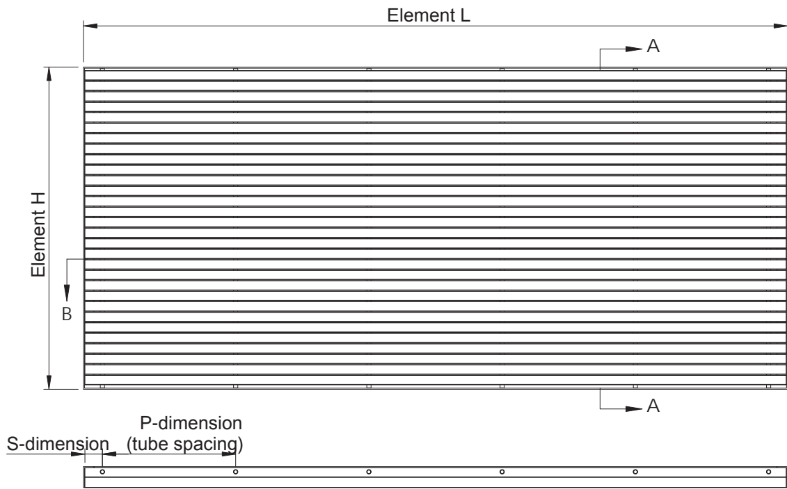
SECTION B-B
