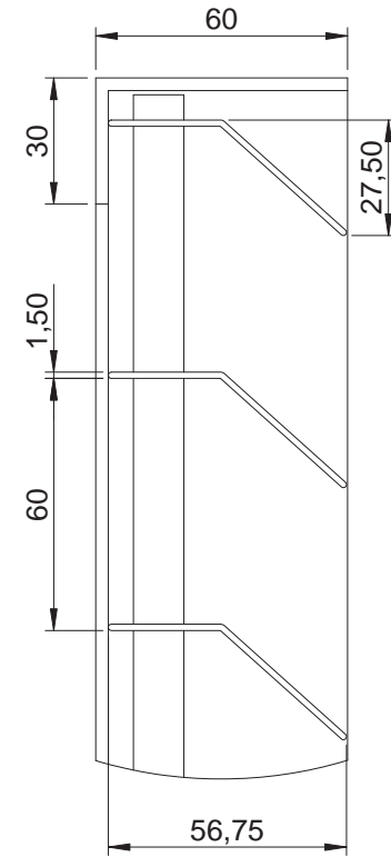
DETAIL C SCALE 1 : 2
