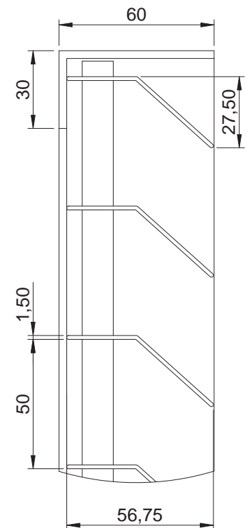
DETAIL C SCALE 1 : 2
