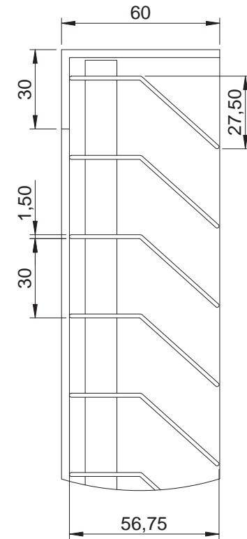
DETAIL C SCALE 1 : 2
